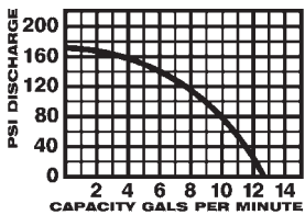
Composite Performance Curve At 0 Lbs Suction Pressure
